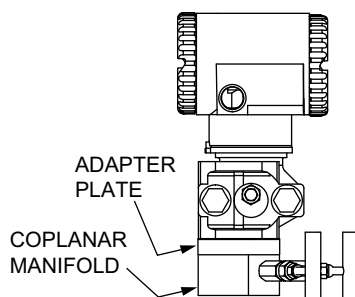
Figure 12 - Low Profile (LP1) Transmitter – Mounted to a Coplanar Manifold using an Optional Adapter Plate
